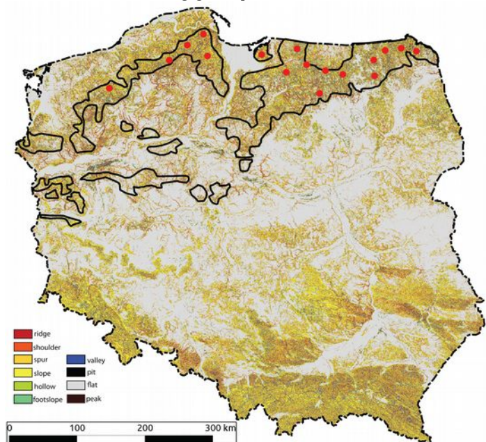
Figure 1. Geomorphometric map (gmphMap) of Poland calculated from the 30m resolution DTM using geomorphons method. Black contours indicate a
